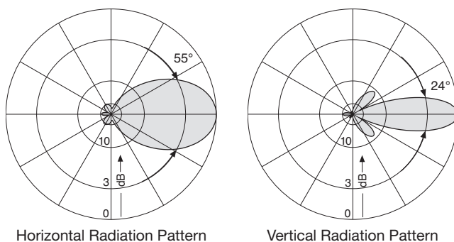
Horizontal Radiation Pattern
