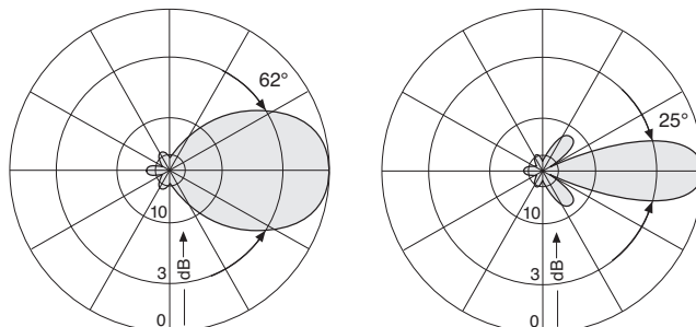
Horizontal Radiation Pattern
