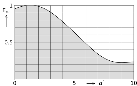
Vertical Radiation Pattern
