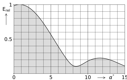
Vertical Radiation Pattern
